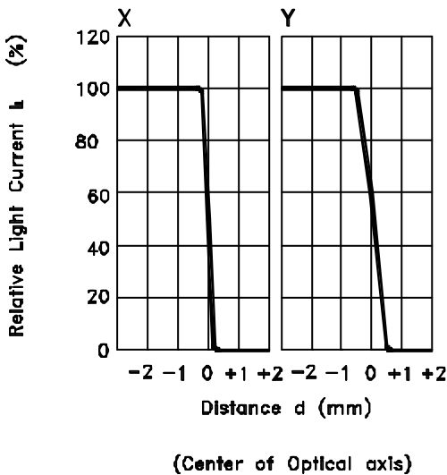
Fig.7 Sensing Position Characteristics (Typical)
