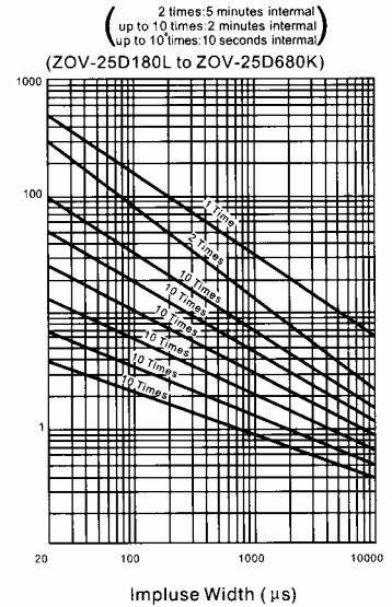
Impulse Lifetime Ratings
