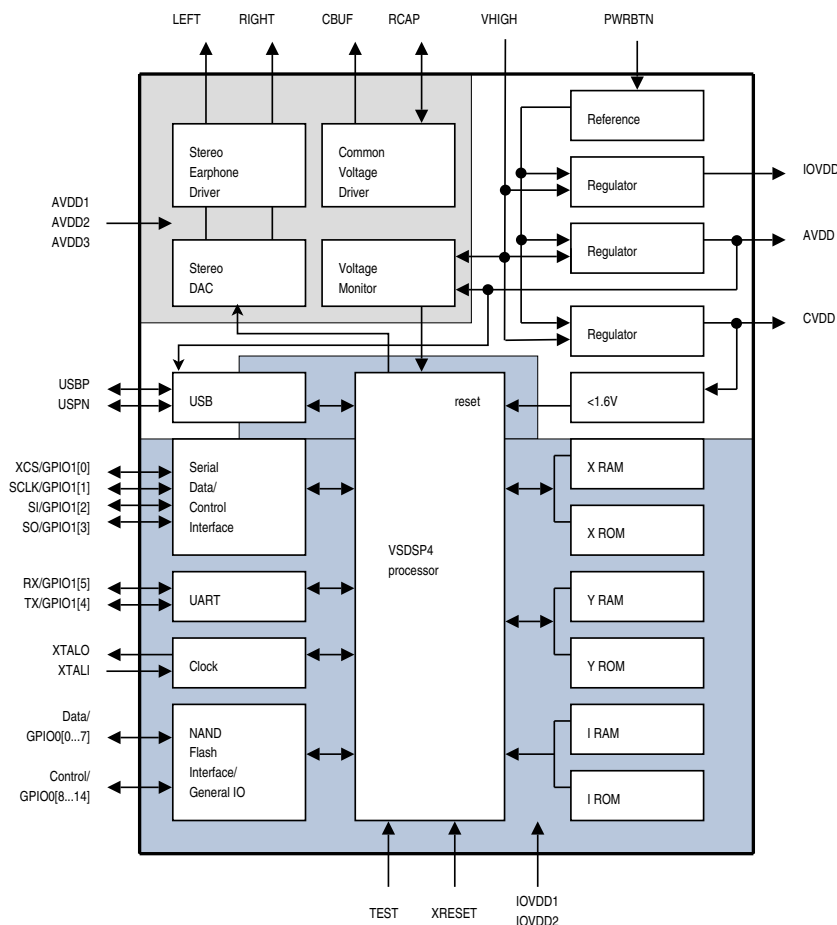
Figure 2: VS1000 Block Diagram
