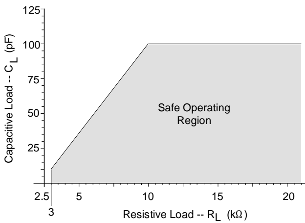
Figure 16. Maximum Loading
