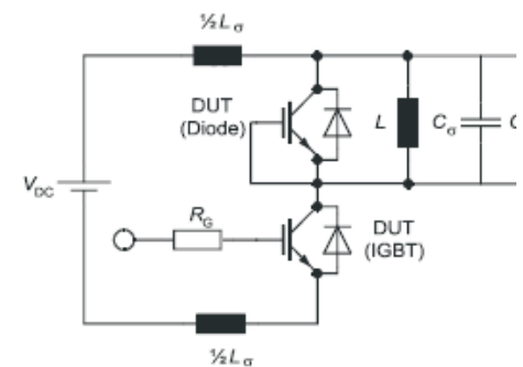
Figure E. Dynamic test circuit Parasitic inductance L_{\sigma} , Parasitic capacitor C_{\sigma} , Relief capacitor C , (only for ZVT switching)
