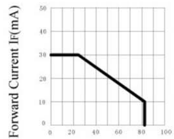
Ambient Temperature TA(°C) Fig.3 Forward Current Derating Curve
