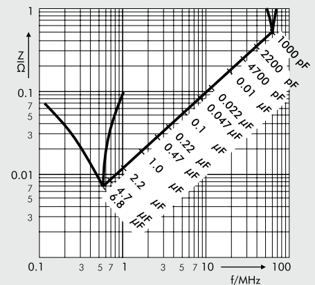
Impedance change with frequency (general guide).
